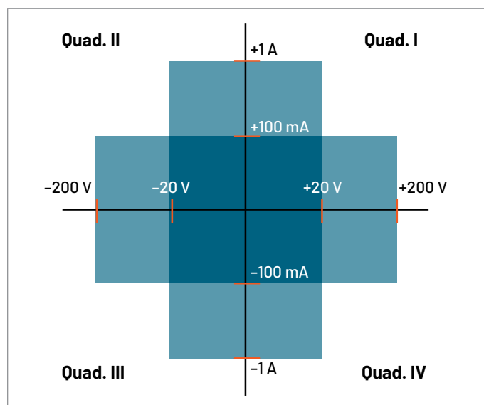
2450 power envelope.
