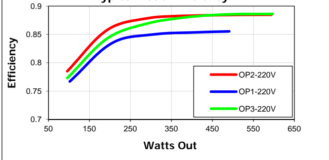
Typical Load Efficiency
