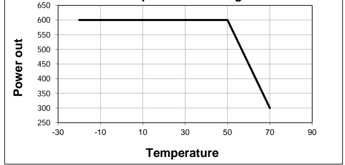
Temperature Derating
