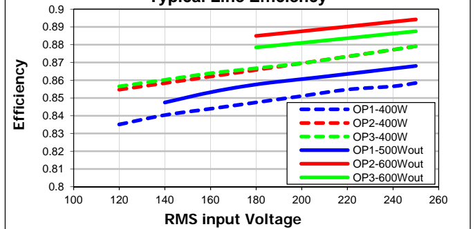
Typical Line Efficiency
