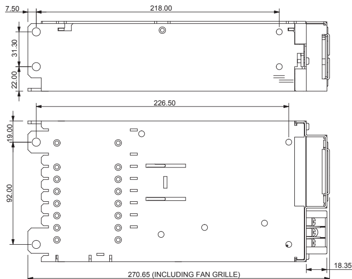
Screw & Fast-on Terminal Case
