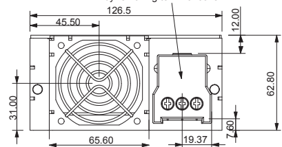
Screw & Fast-on Terminal Case
