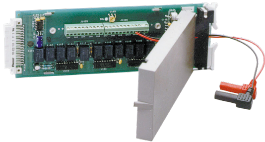
2000-SCAN 10-Channel Multiplexer.
