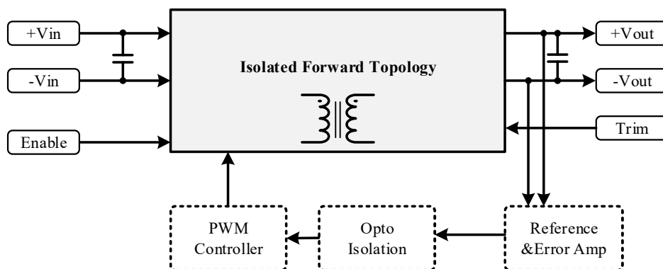
SHBF Series Block Diagram
